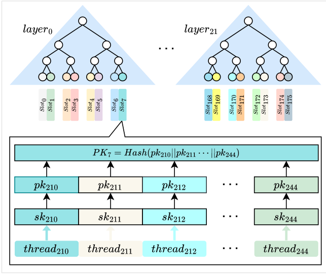
Fig. 7. The key pair generation of WOTS + .
