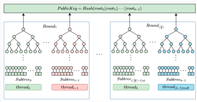
Fig. 6. Parallel strategy for FORS.
