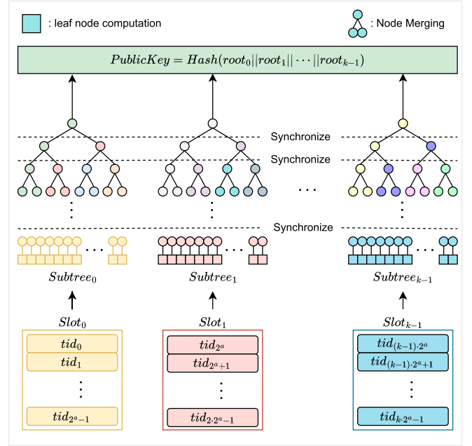
Fig. 8. Low latency parallel strategy for FORS.
