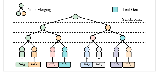
Fig. 3. Parallel strategy for Merkle tree.
