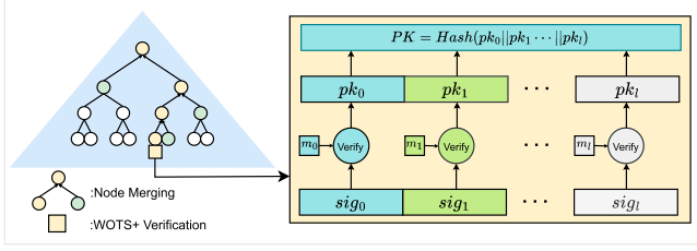
Fig. 9. The verification of MSS in hypertree.
