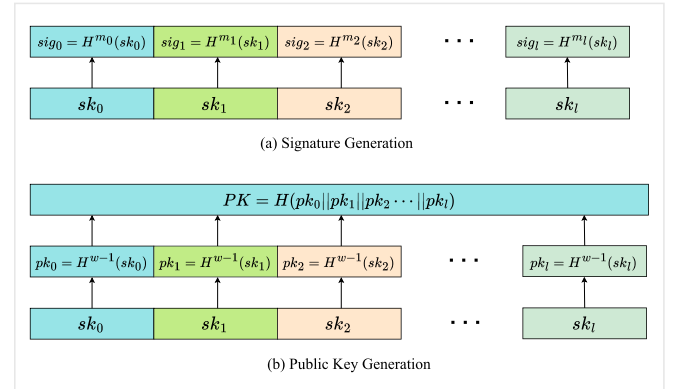
Fig. 4. Computation process of WOTS + .
