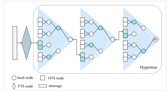
Fig. 2. An overview of SPHINCS + structure with h = 9 and d = 3 .
