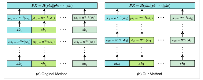
Fig. 10. Comparison of the original method and our method.
