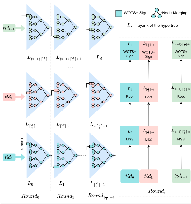
Fig. 5. Parallel strategy for hypertree.
